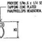
BRASS CUTLERY CLIP SCALE 1:1
