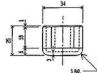
ELEVATION - DRINKER 2 OFF REQ'D. SCALE 1:1
