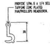
30 BRASS BOX HOOK SCALE 1:1
