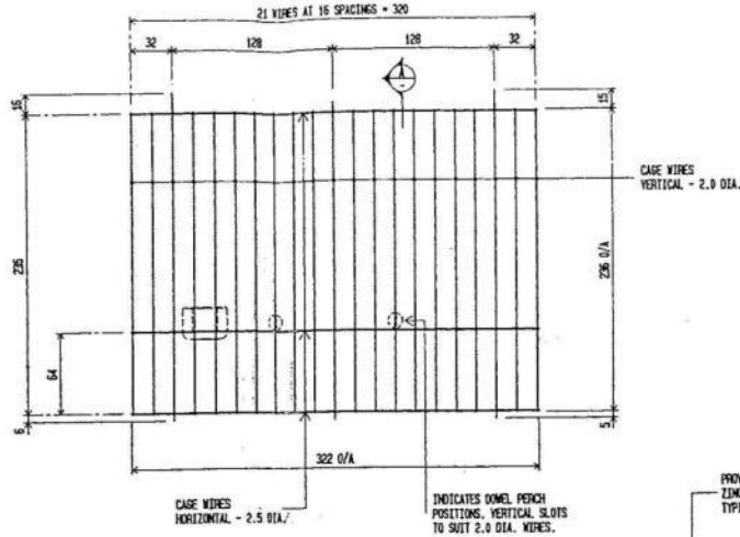
ELEVATION - WIRE CAGING NOTE: CASE WIRES - 2.0 DIA. / 2.5 DIA. TO BE CHROMIUM PLATED IN ACCORDANCE WITH SHOWCASE SPECIFICATION.
